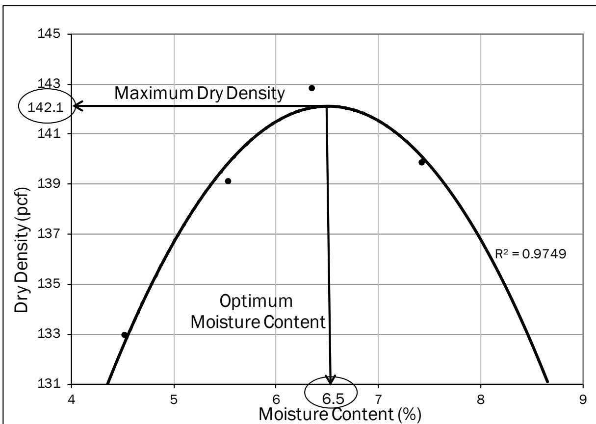
Figure A3: Tex-113-E, Moisture-Density Curve
