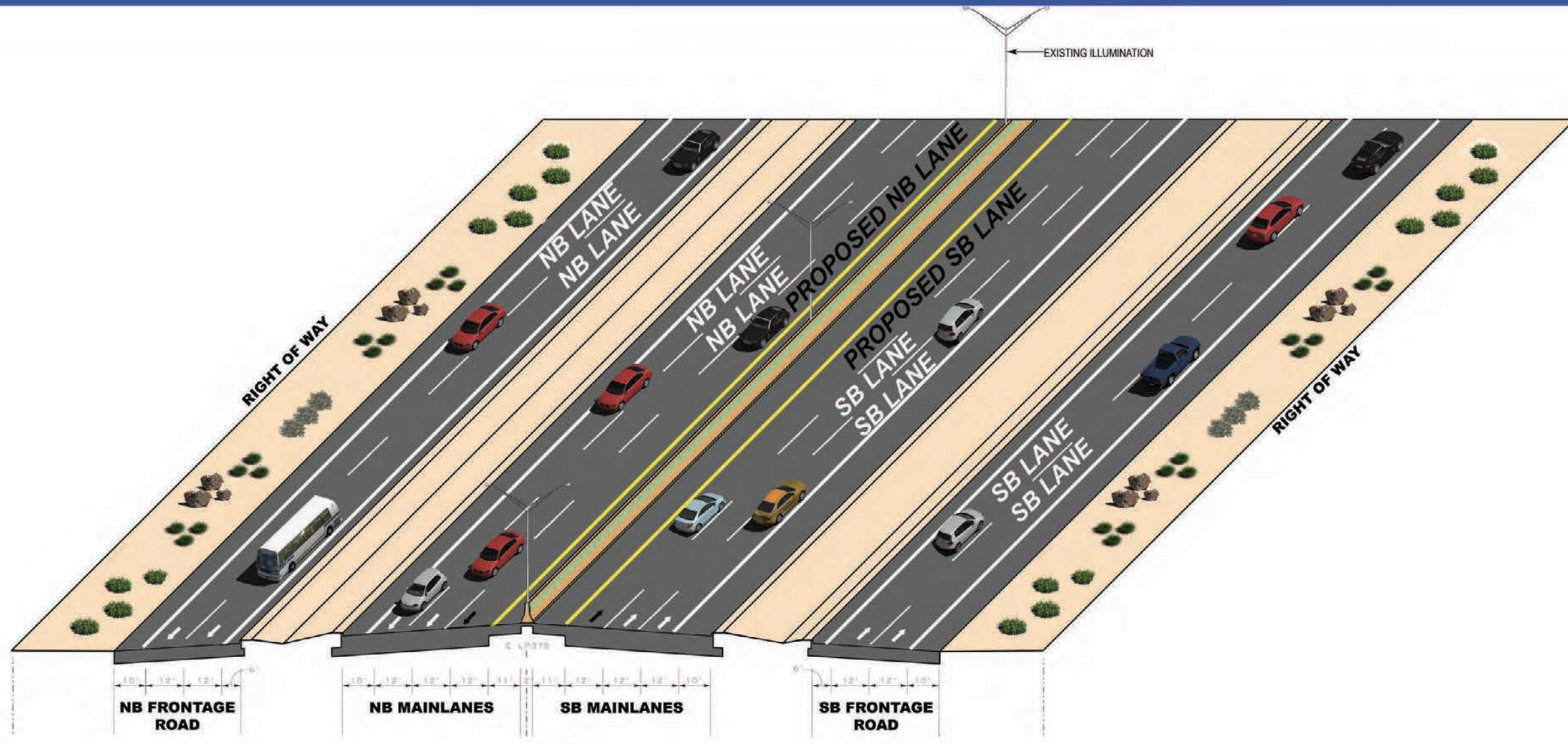
PROPOSED LOOP 375 TYPICAL SECTION
