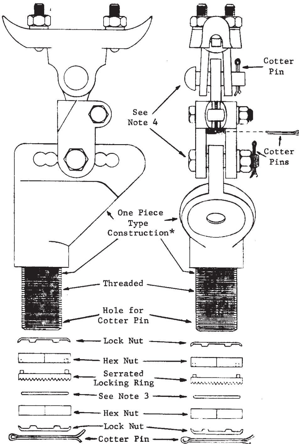
Serrated Locking Ring-Detail
