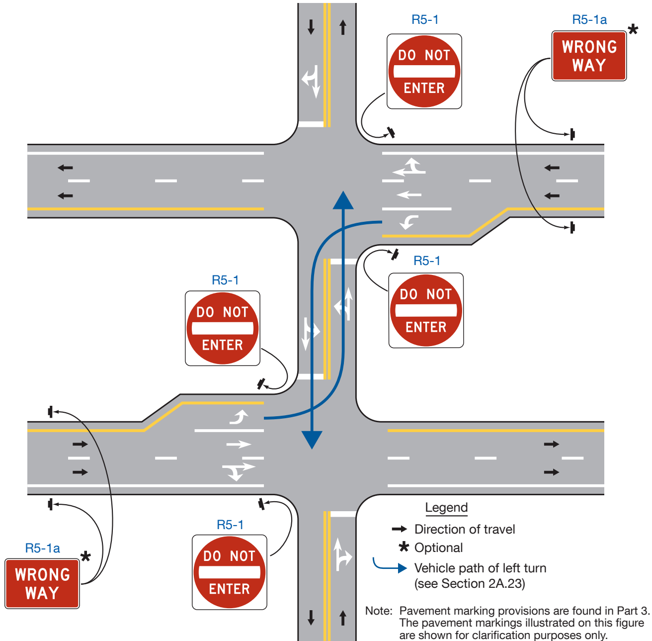
Figure 2B-14. Locations of DO NOT ENTER and WRONG WAY Signage for Divided Highway Crossings that Function as Two Separate Intersections
