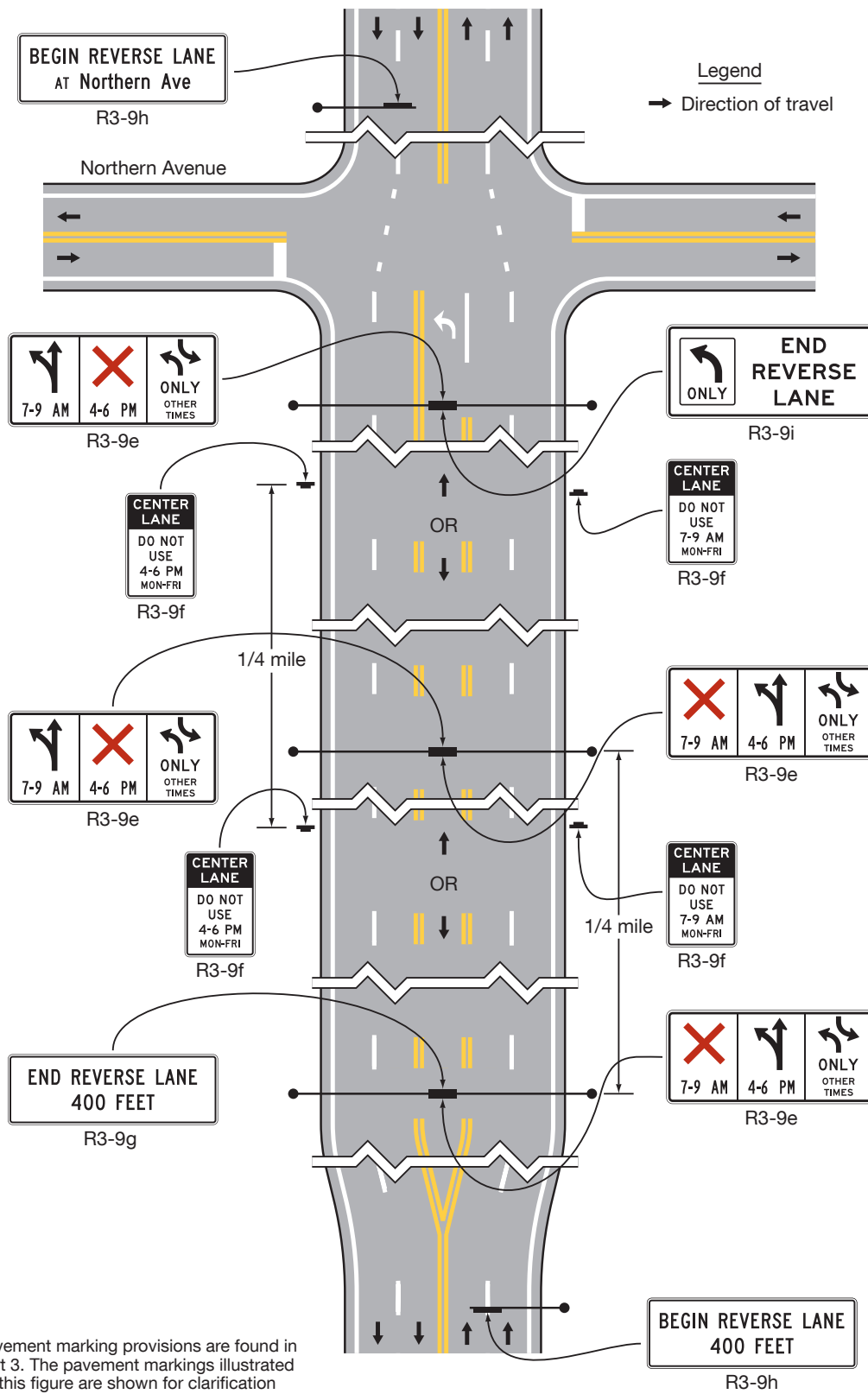
Figure 2B-7. Location of Reversible Two-Way Left-Turn Signs
