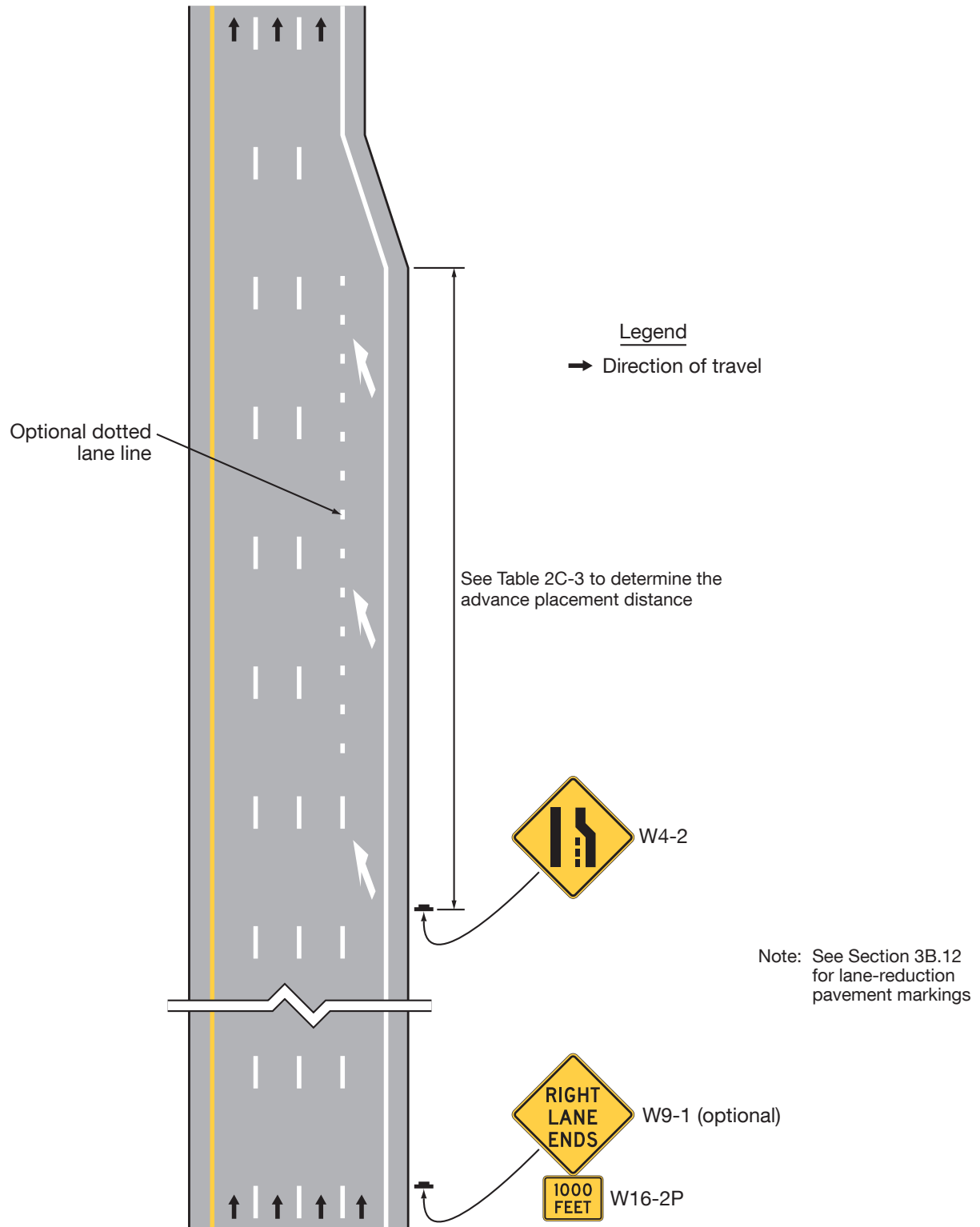
Figure 2C-13. Example Sequences for Lane Ends and Lane Merge Signs (Sheet 1 of 5)
