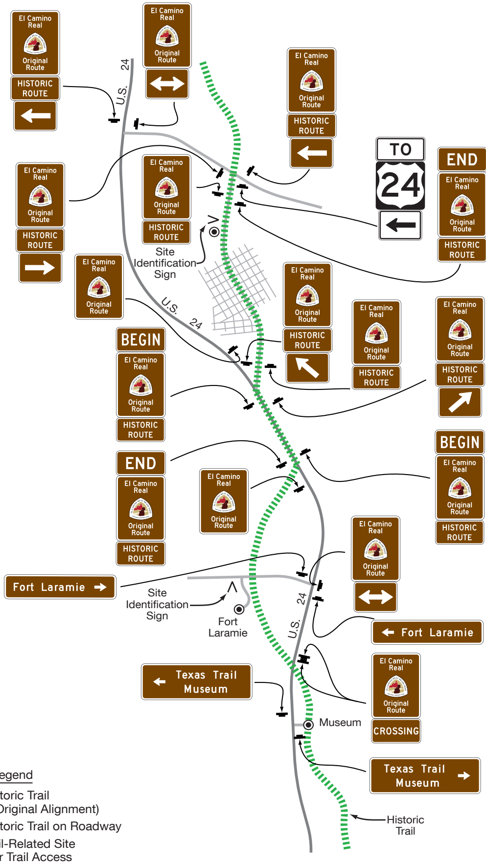
Figure 2D-35. Example of Guide and Directional Signing for a National Historic Trail
