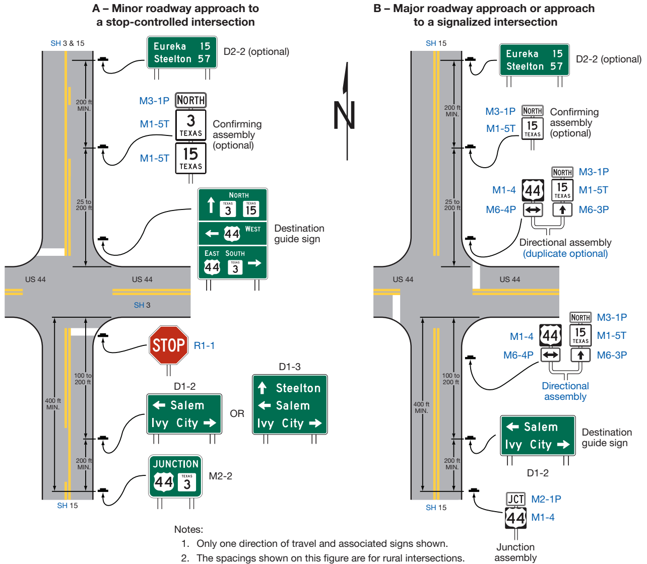
Figure 2D-7. Examples of Consolidation of Route Sign Assemblies into Guide Signs (Sheet 1 of 2)
