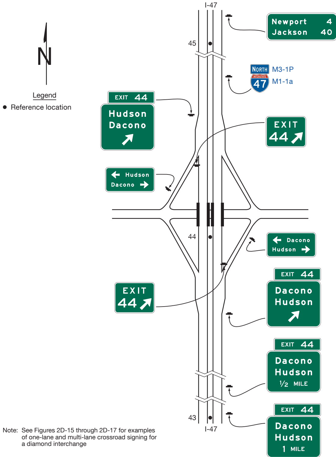
Figure 2E-27. Example of Guide Signs for a Diamond Interchange
