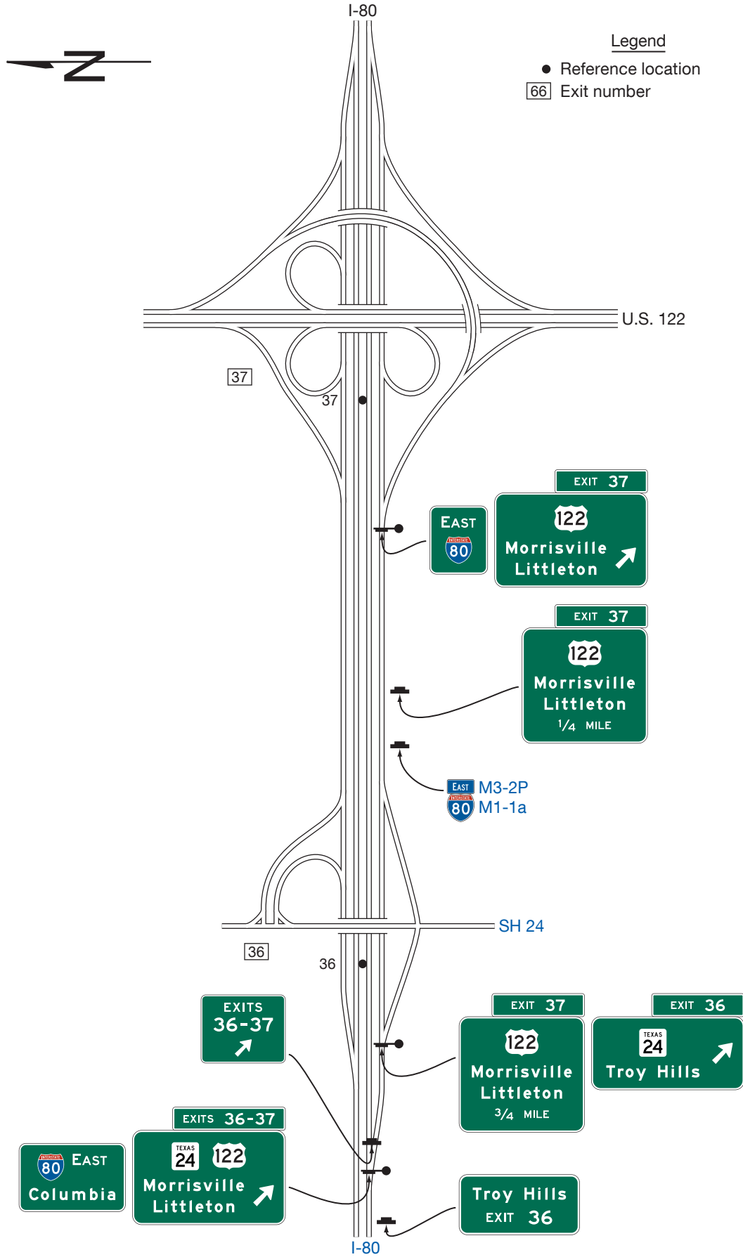
Figure 2E-32. Examples of Guide Signs for Successive Interchanges with Collector-Distributor Roadways (Sheet 1 of 2)
