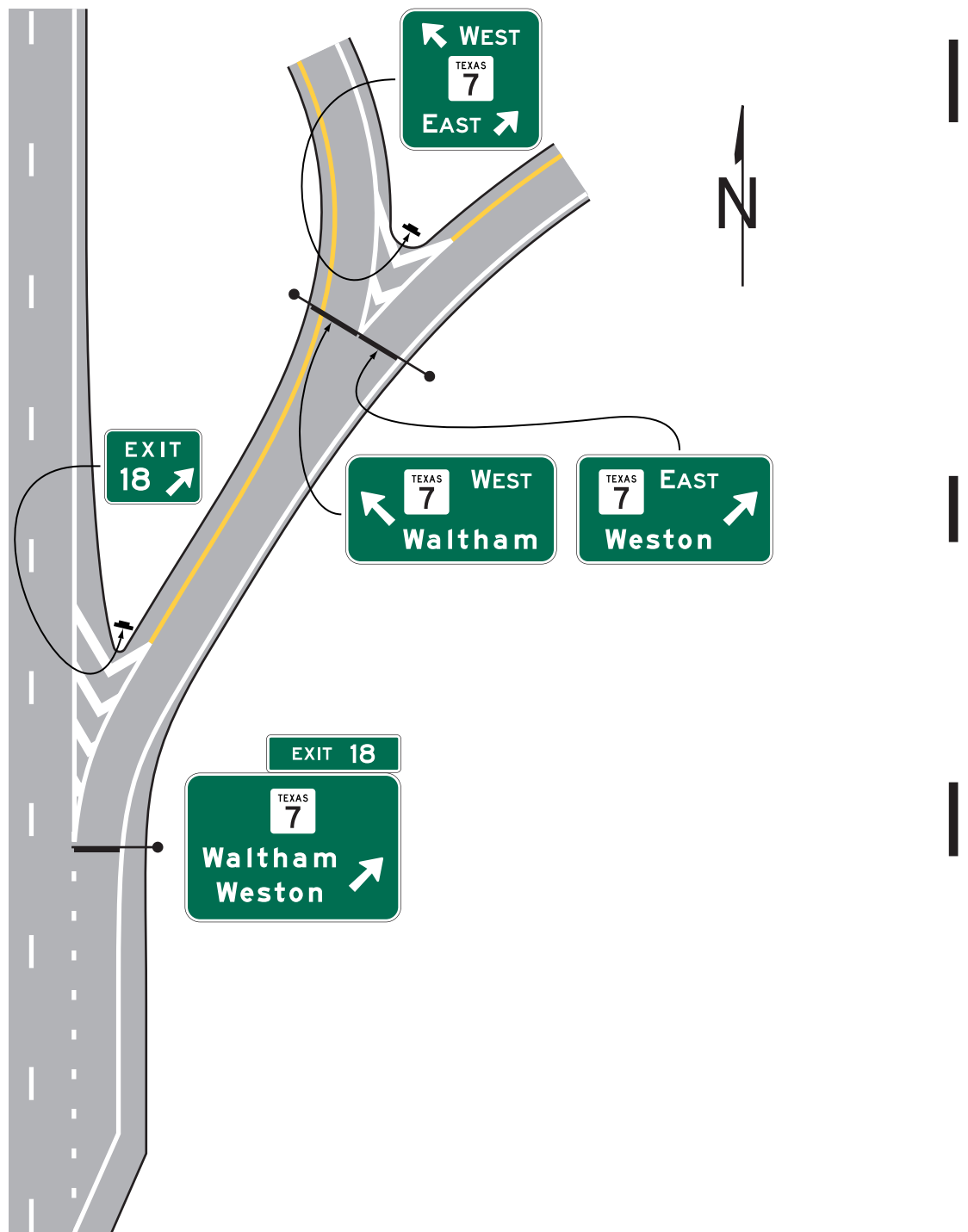
Figure 2E-25. Examples of Signing for an Interchange Exit Ramp with a Downstream Split (Sheet 1 of 2)
