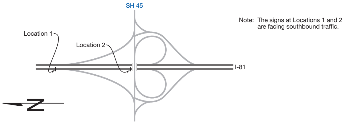
A – Before sign spreading
