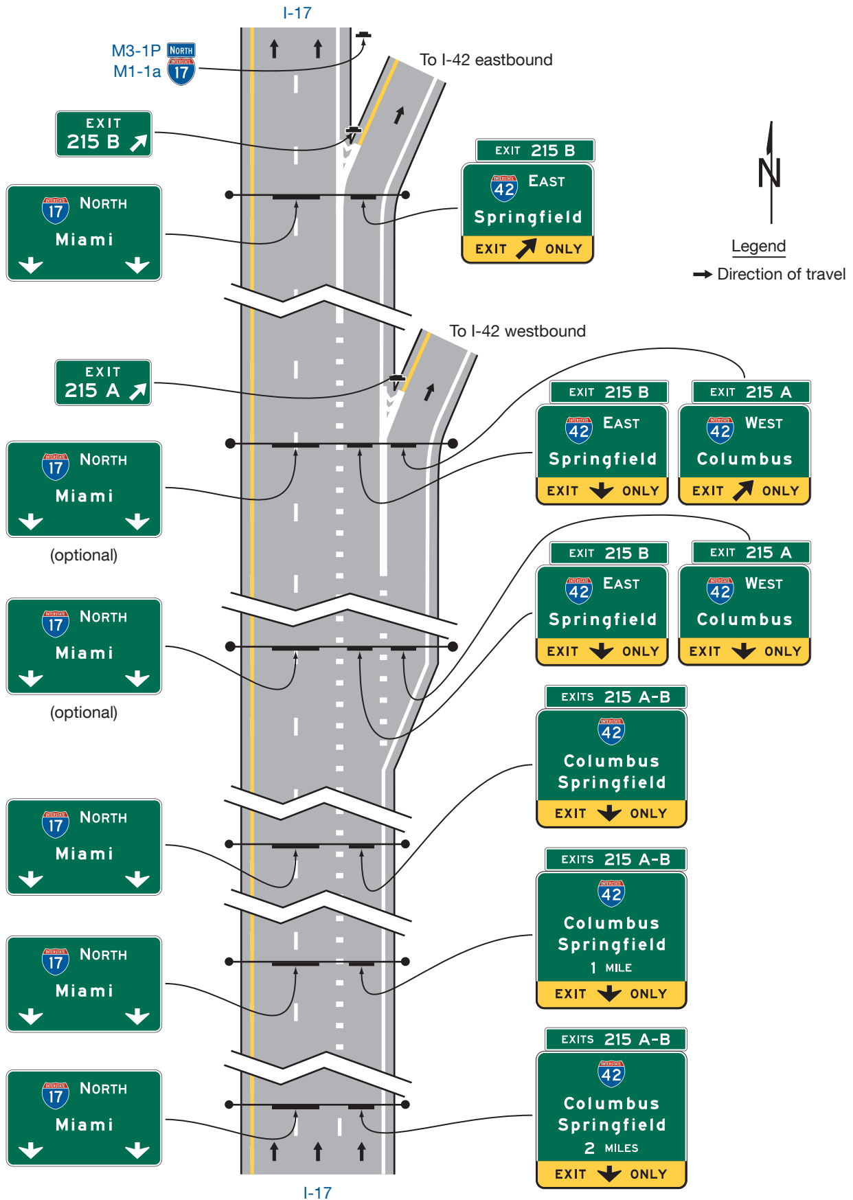
Figure 2E-33. Examples of Guide Signs for a Freeway-to-Freeway Interchange (Sheet 2 of 2)
