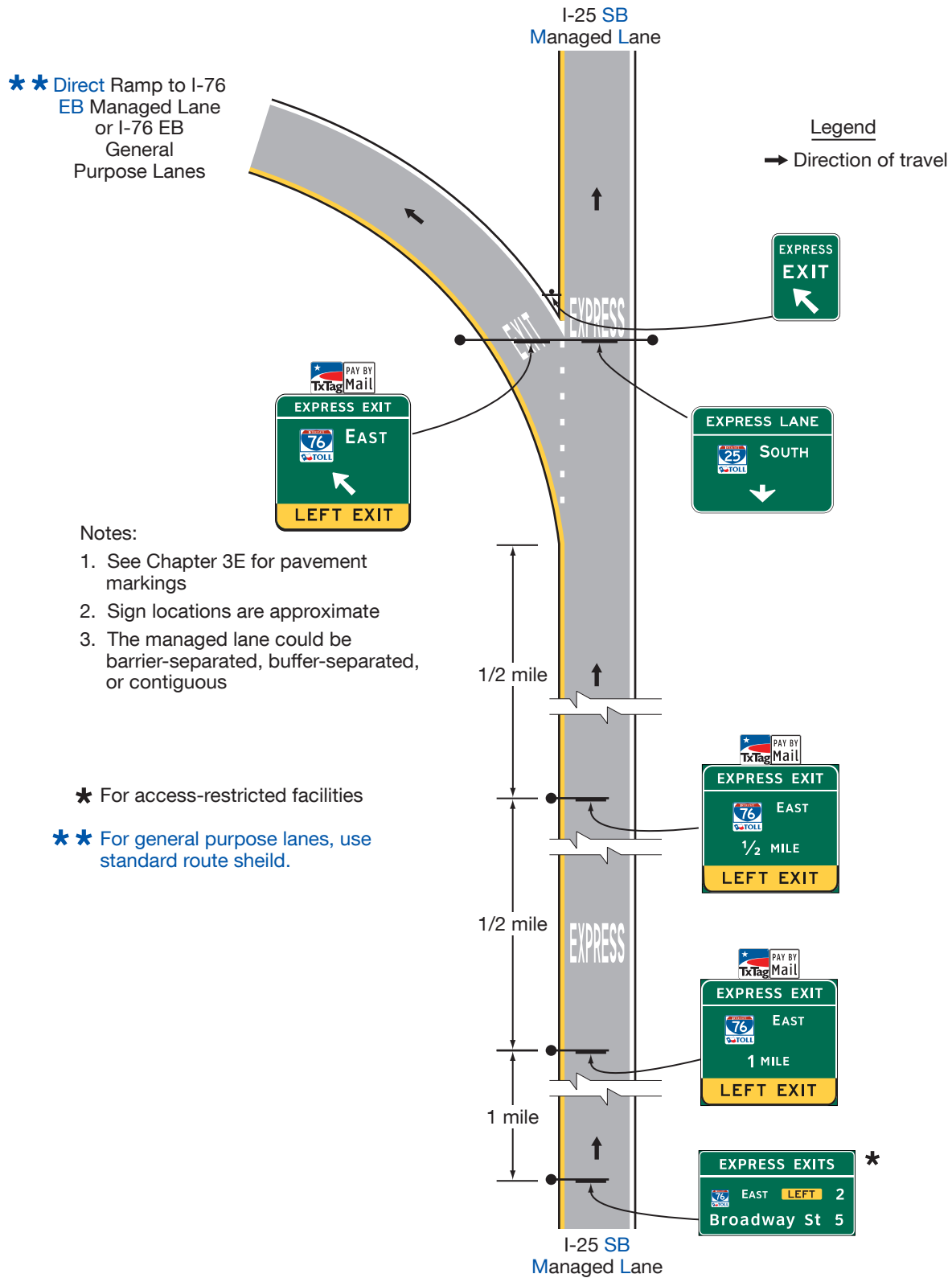
Figure 2G-29. Examples of Guide Signs for a Direct Access Ramp between Managed Lanes on Separate Freeways
