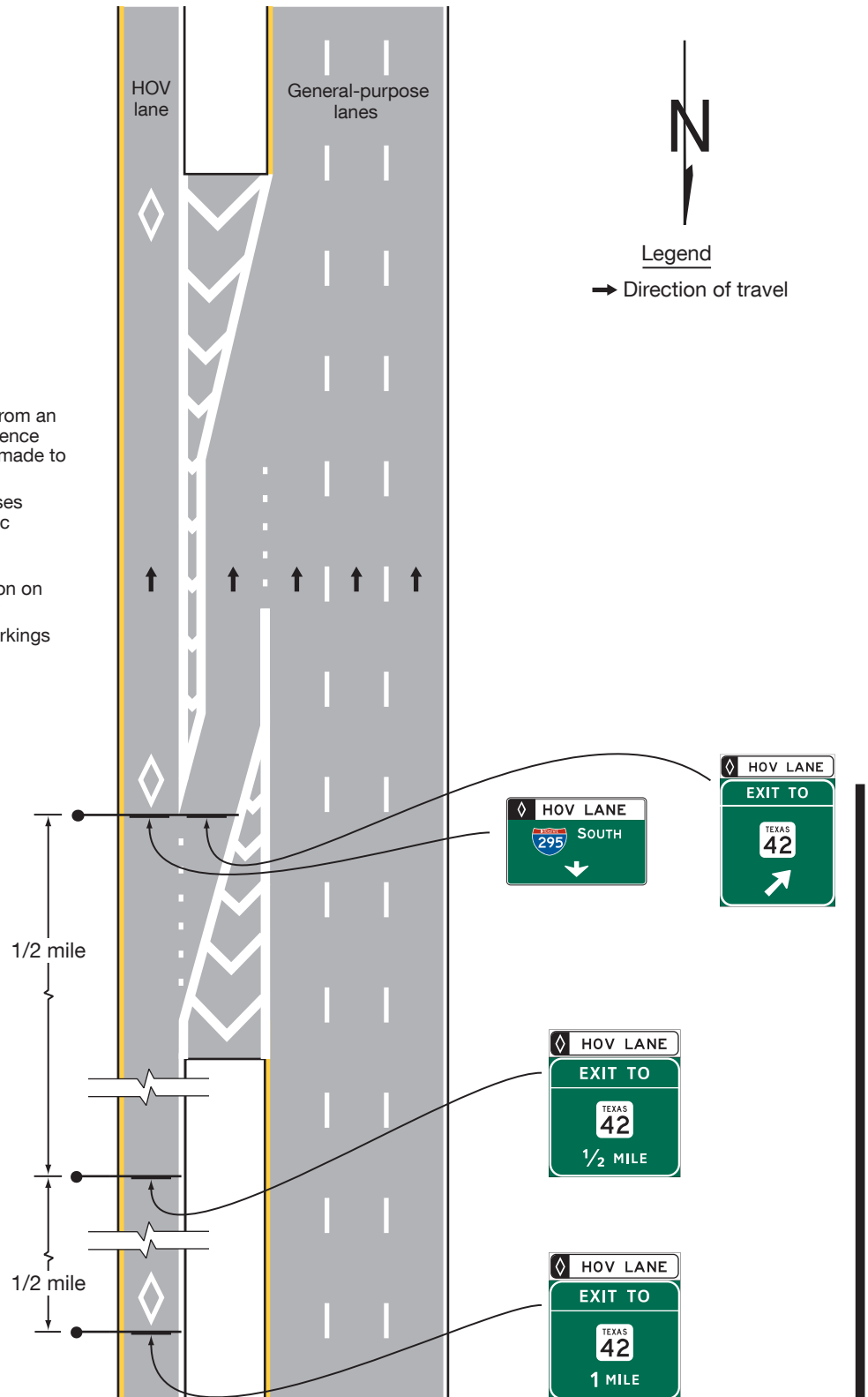
Figure 2G-13. Examples of Signs for an Intermediate Egress from a Barrier-Separated or Buffer-Separated HOV Lane
