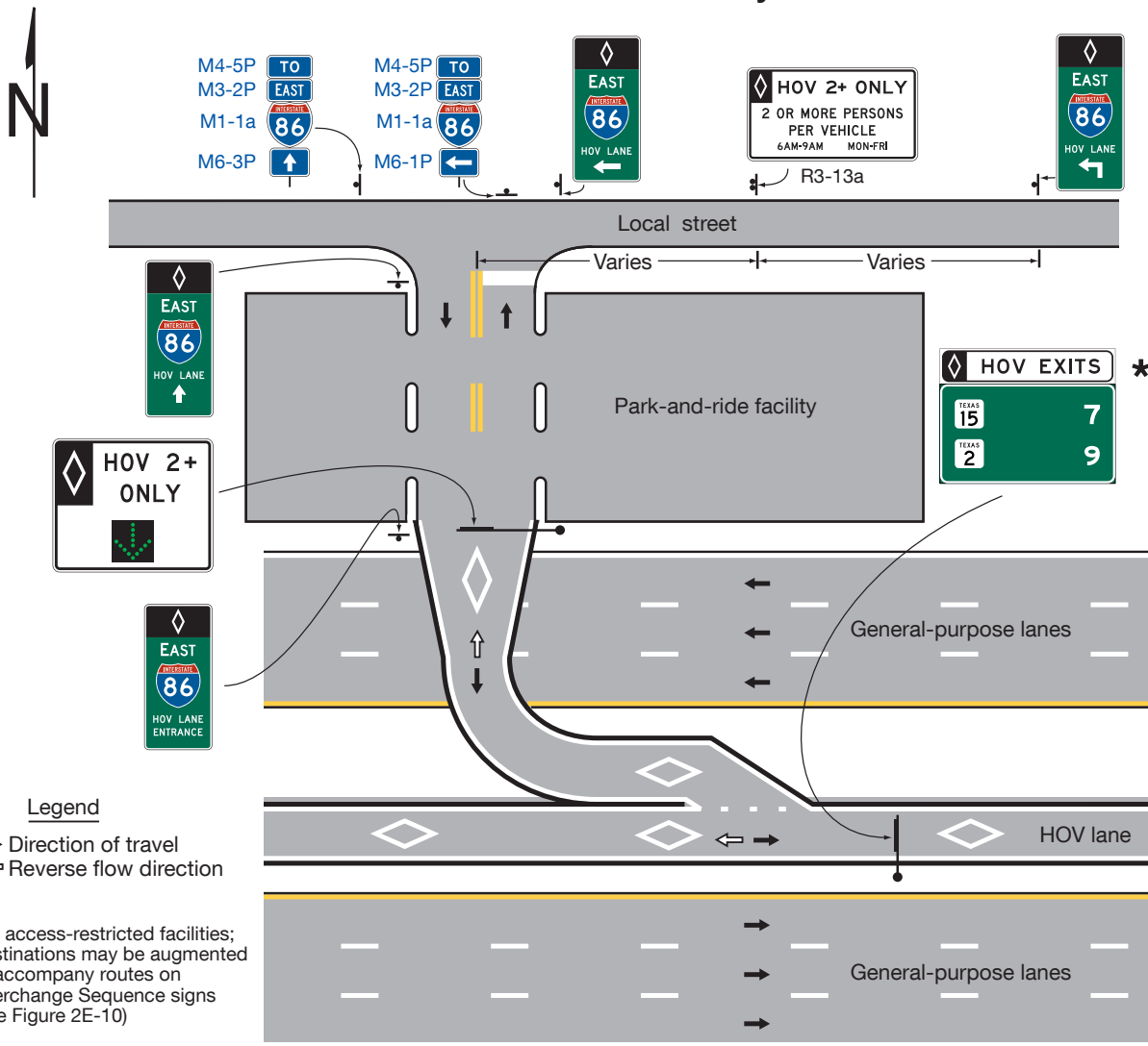
Figure 2G-14. Example of Signing for a Direct Entrance Ramp to an HOV Lane from a Park-and-Ride Facility and a Local Street
