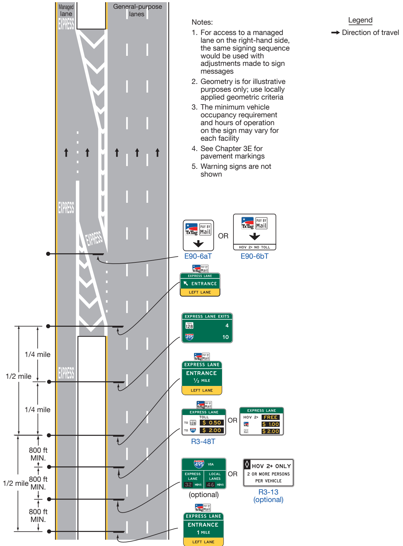
Figure 2G-23. Example of Signing for an Intermediate Entry to a Barrier- or Buffer-Separated Priced Managed Lane
