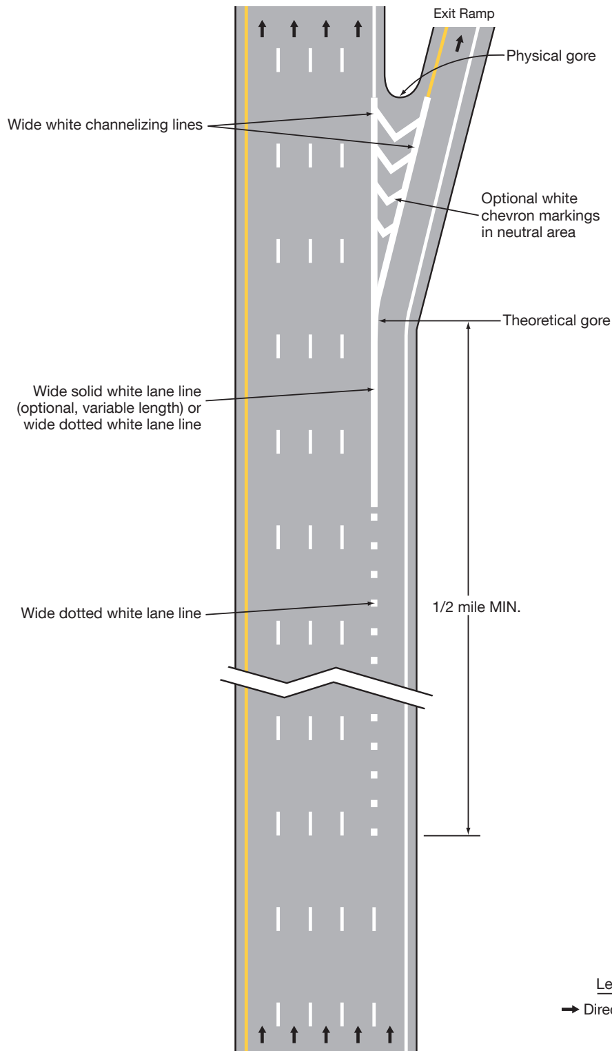
A – Lane drop at a single lane exit ramp
