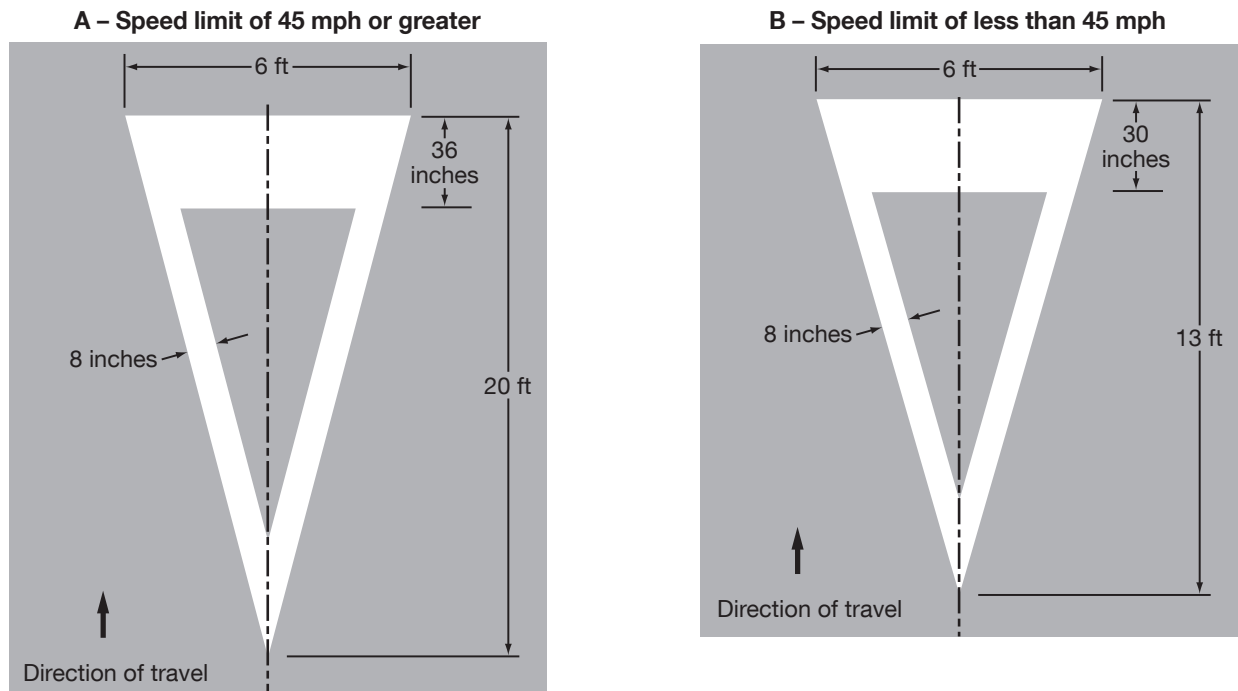
Figure 3B-20. Yield Ahead Triangle Symbols
