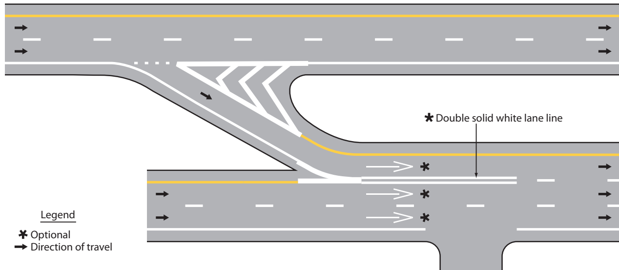
Figure 3B-8. Example of Double Solid White Line Used to Prohibit Lane Changing
