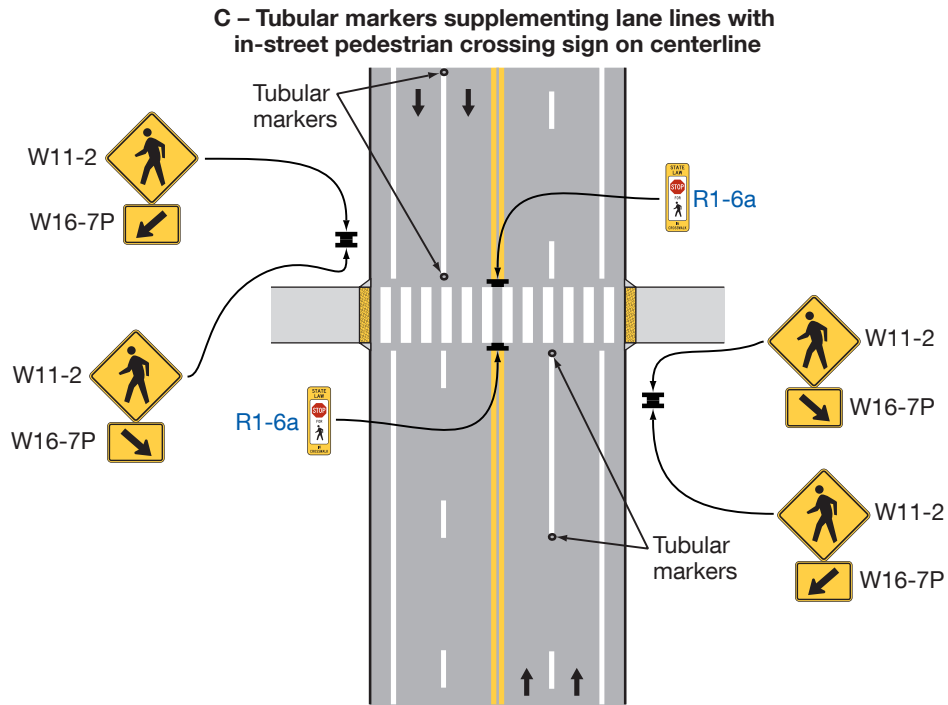
Figure 3I-1. Examples of Tubular Markers Supplementing Pavement Markings in Advance of an Unsignalized Crosswalk (Sheet 2 of 2)
