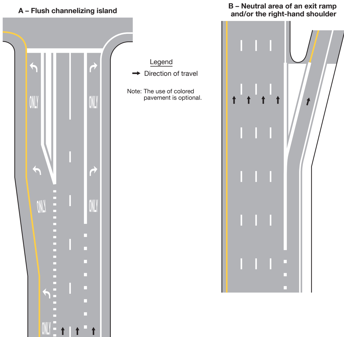
Figure 3H-3. Examples of White-Colored Pavement Applications
