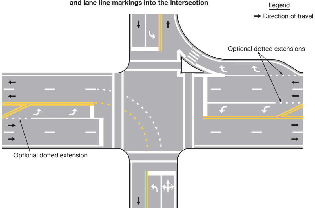
D – Typical dotted line markings to extend center line and lane line markings into the intersection
