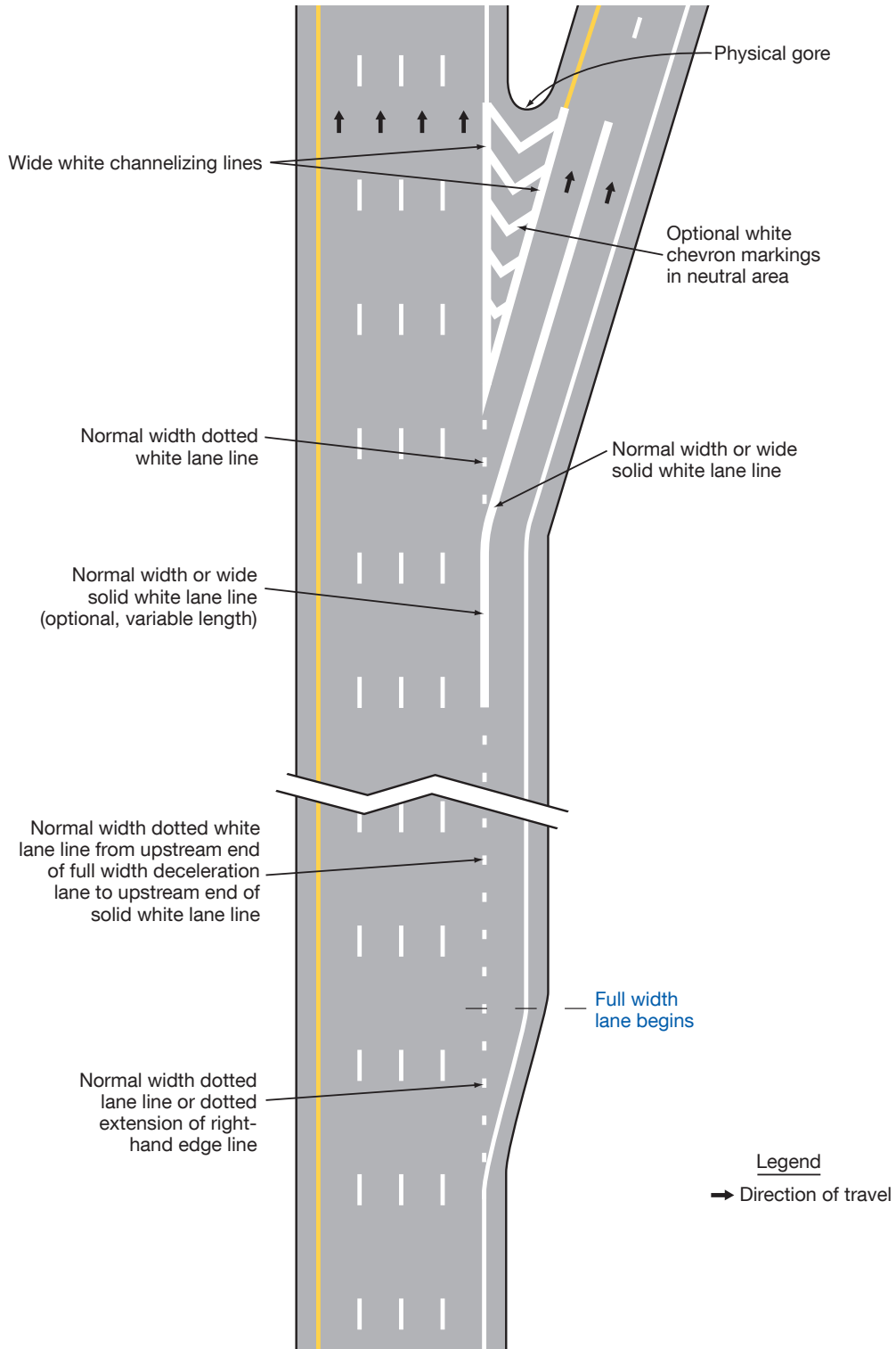
C – Parallel deceleration lane at a multi-lane exit ramp having an optional exit lane that also carries the through route
