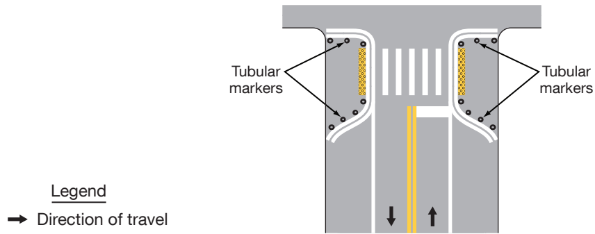
A – Sidewalk extension to reduce the pedestrian crossing distance
