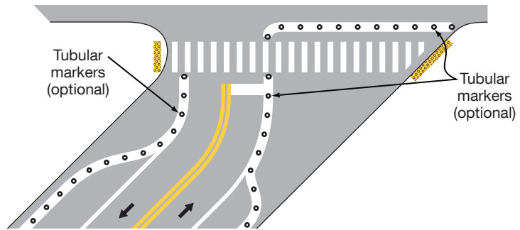
B – Channelizing for speed control and altered travel paths
