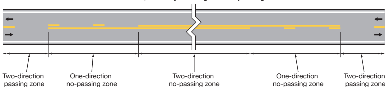
B – Two-lane, two-way marking with no-passing zones
