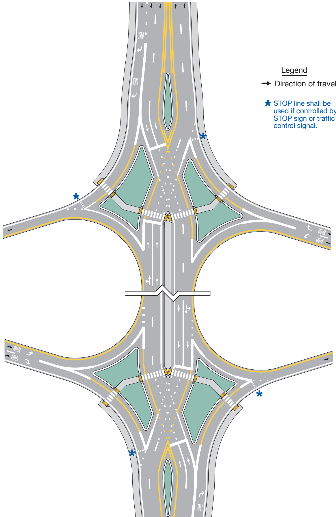
Figure 3B-29. Example of Pavement Markings for a Diamond Interchange with a Transposed Alignment Crossroad
