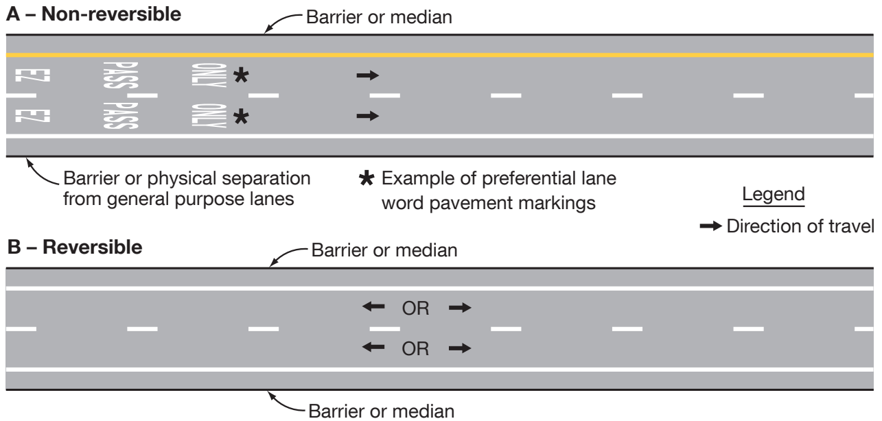
Figure 3E-1. Markings for Barrier-Separated Preferential Lanes
