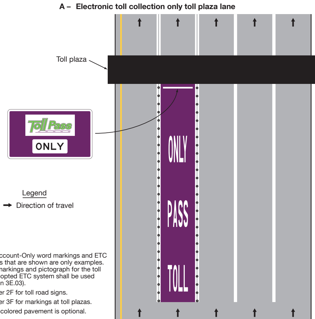
Figure 3H-6. Examples of Purple-Colored Pavement Applications (Sheet 1 of 2)
