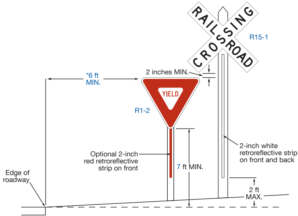
Figure 8B-3. Crossbuck Assembly with a YIELD or STOP Sign on a Separate Sign Support
