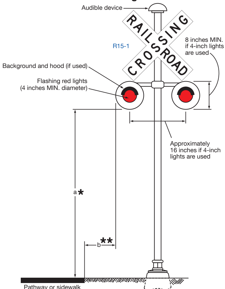
Figure 8E-7. Example of a Flashing-Light Signal Assembly at a Pathway or Sidewalk Grade Crossing
