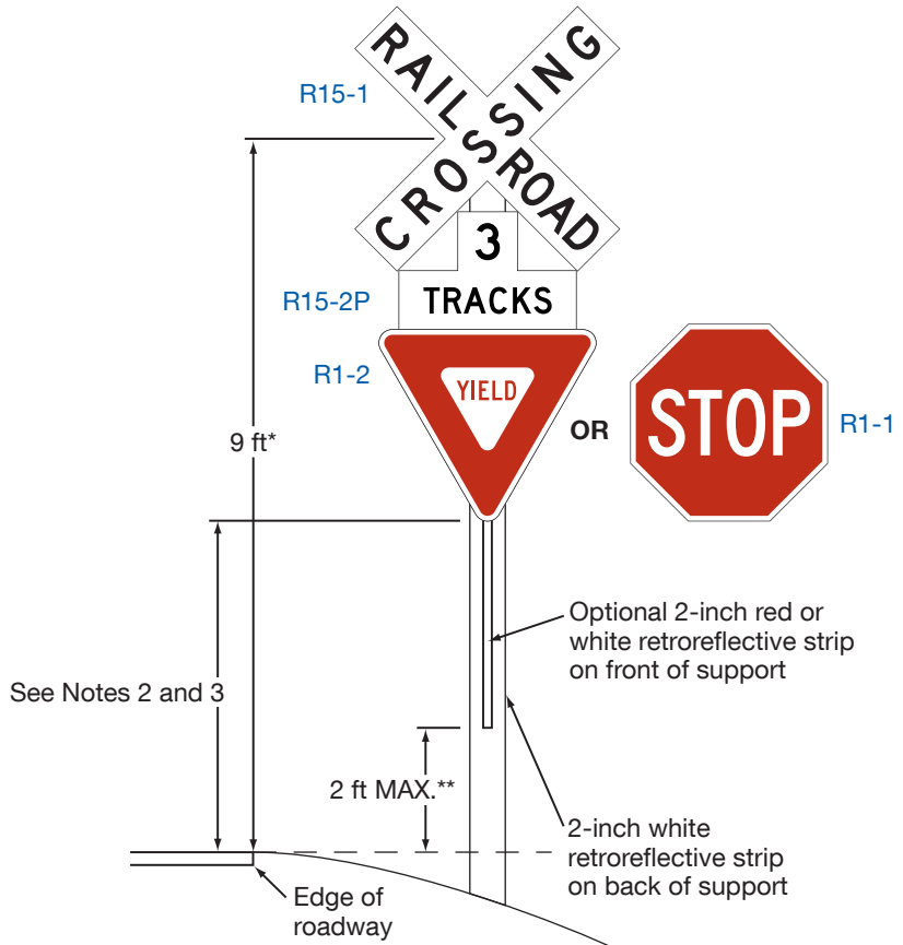
Figure 8B-2. Crossbuck Assembly with a YIELD or STOP Sign on the Crossbuck Sign Support
