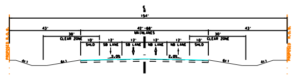
C PROPOSED US 83-84 TYPICAL SECTION SOUTH OF Y-INTERSECTION
