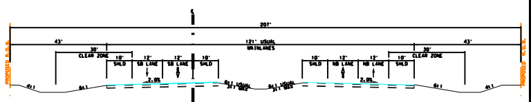
B PROPOSED US 83-84 TYPICAL SECTION NORTH OF Y-INTERSECTION
