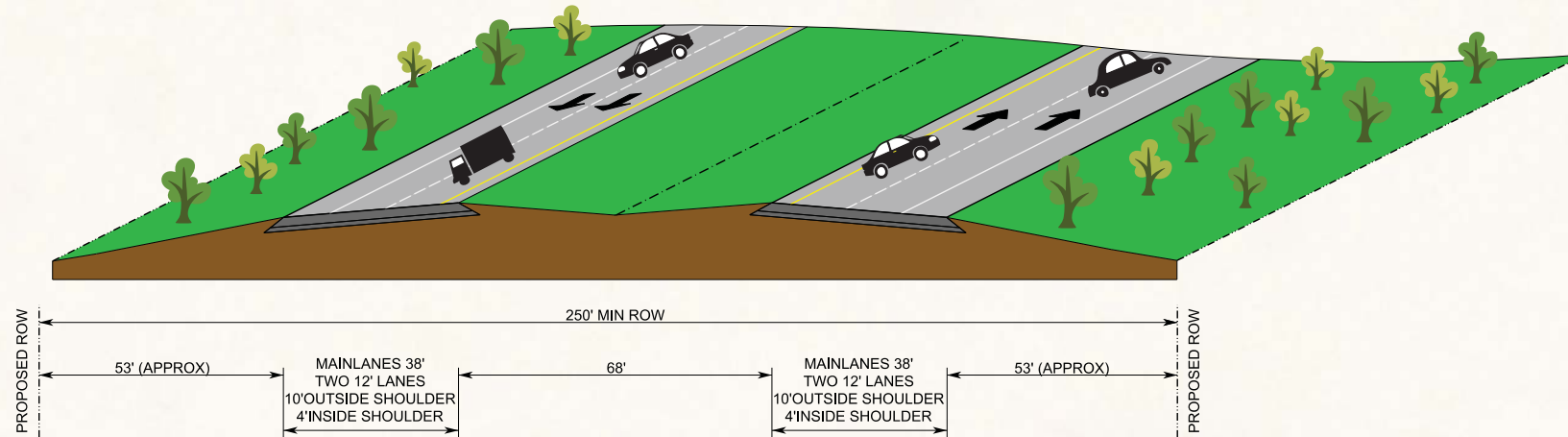
RURAL TYPICAL SECTION WITHOUT ACCESS ROADS
