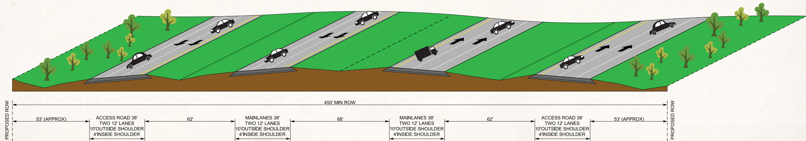
RURAL TYPICAL SECTION WITH ACCESS ROADS
