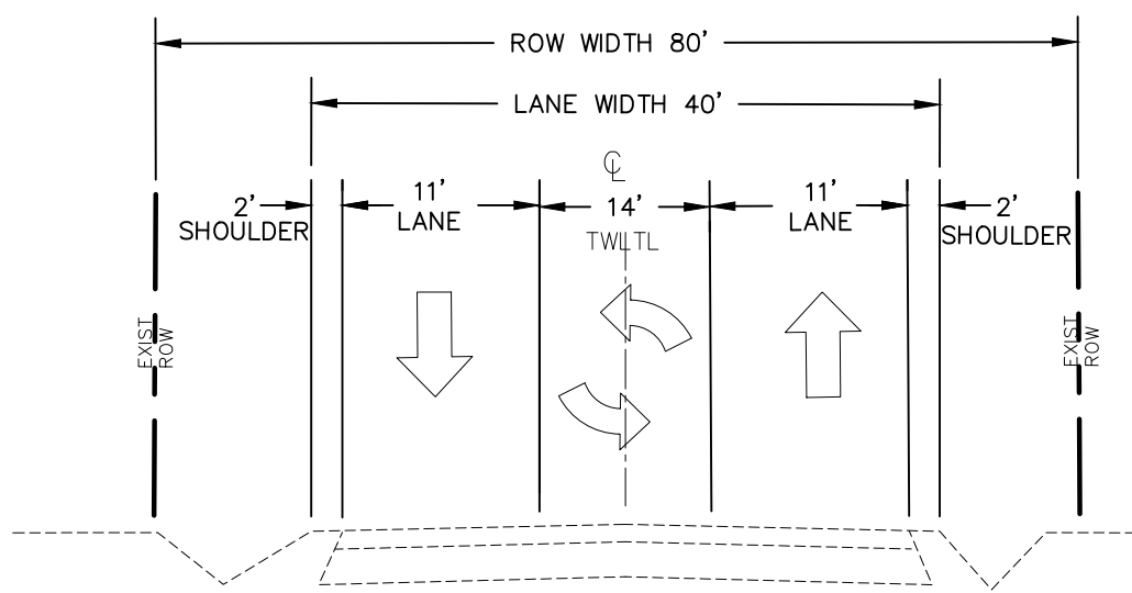
FM 1409 - EXIST TYPICAL SECTION STA 68+50 TO STA 74+00
