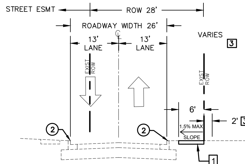
CLEVELAND STREET - PROP TYPICAL SECTION
