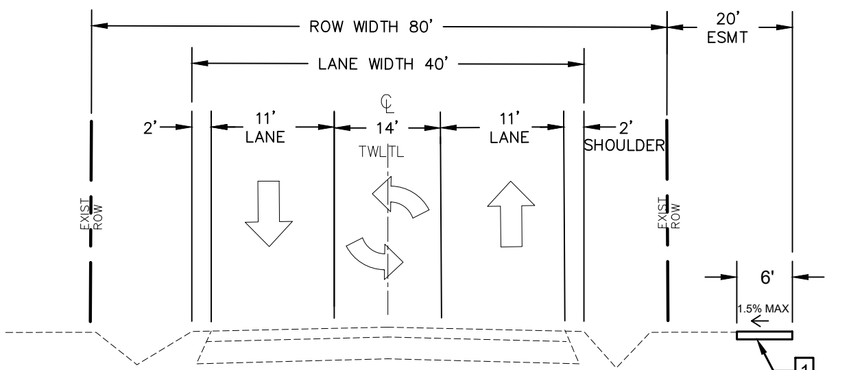
FM 1409 - PROP TYPICAL SECTION STA 68+50 TO STA 74+00
