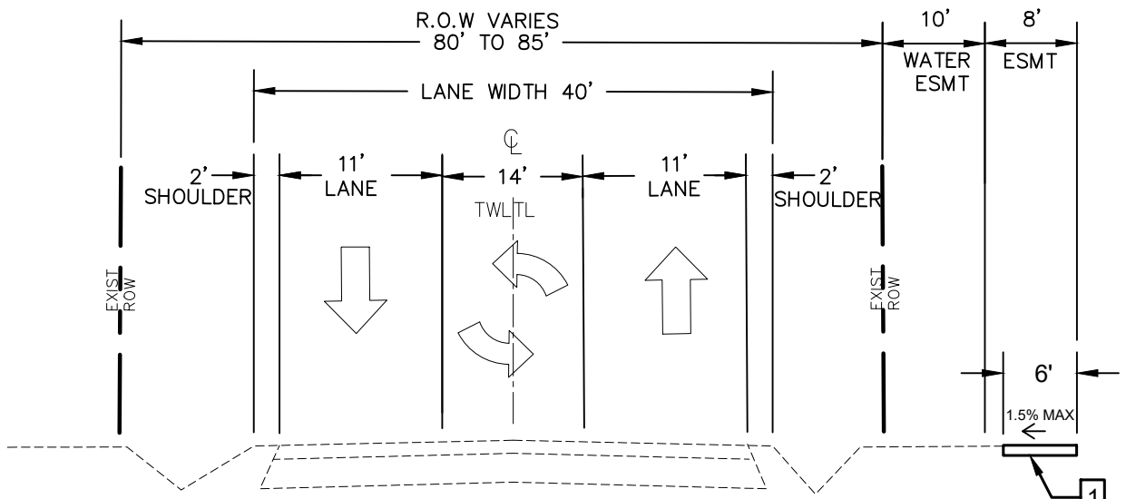
FM 1409 - PROP TYPICAL SECTION STA 64+00 TO STA 68+50
