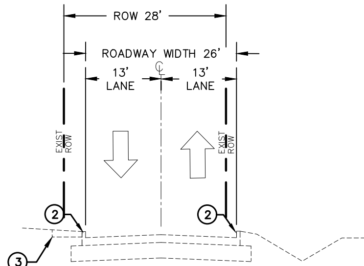
CLEVELAND STREET - EXIST TYPICAL SECTION
