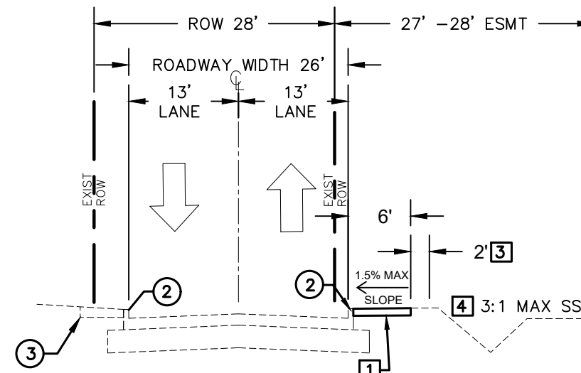
CLEVELAND STREET - PROP TYPICAL SECTION
