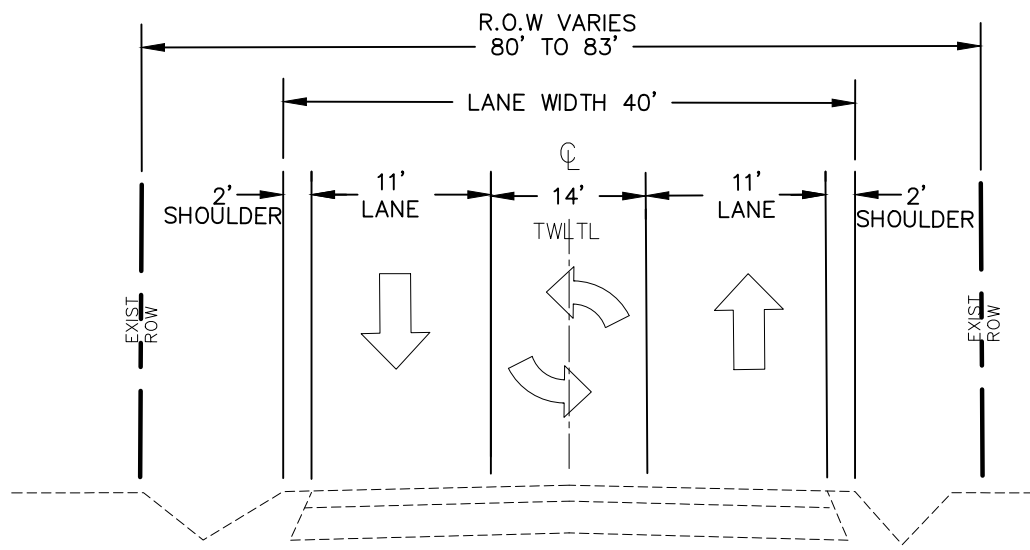
FM 1409 - EXIST TYPICAL SECTION STA 64+00 TO STA 68+50
