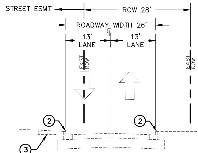
CLEVELAND STREET - EXIST TYPICAL SECTION
