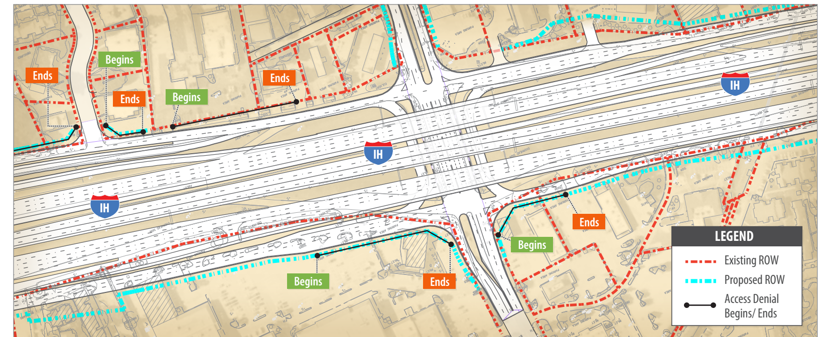
Typical schematic highlighting existing right of way (red line) and proposed right of way line (blue). TxDOT follows state law in seeking to acquire only the property needed for roadway projects. TxDOT also follows established guidelines to control ingress and egress from adjacent properties, also known as control of access.
