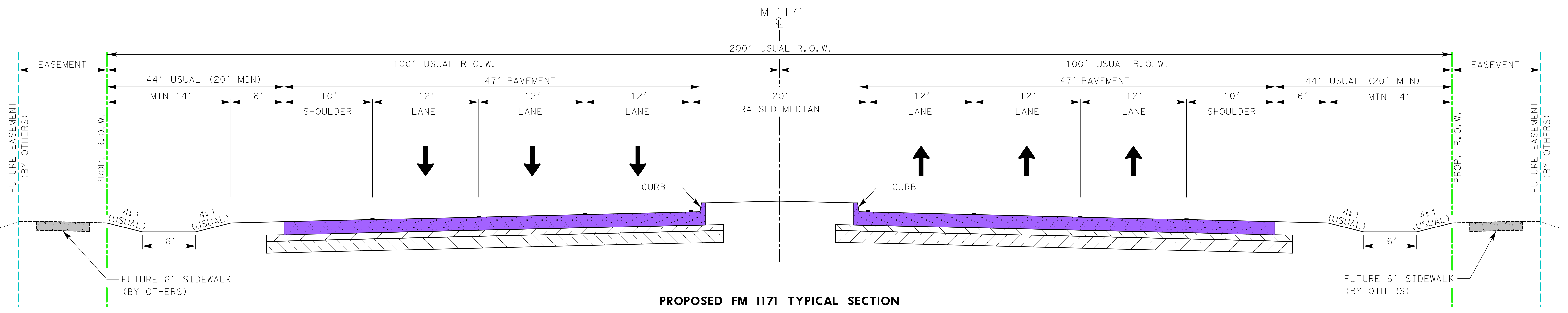
PROPOSED FM 1171 TYPICAL SECTION HARMONSON RD TO IH 35W
