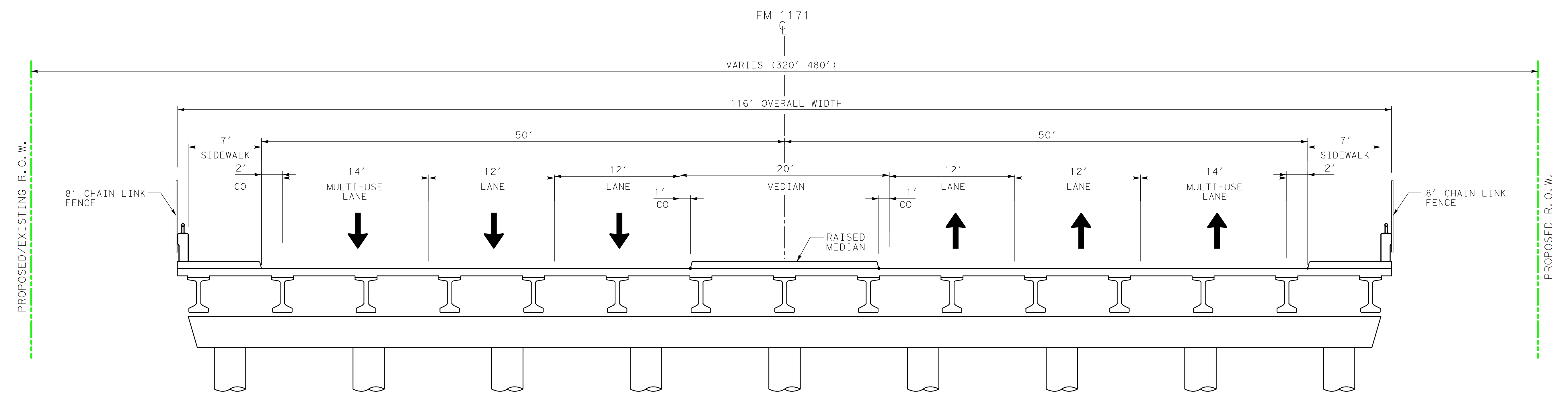
PROPOSED FM 1171 BRIDGE SECTION OVER FM 156, B.N.S.F RAILROAD, GE TEST TRACK & CEMETERY RD.
