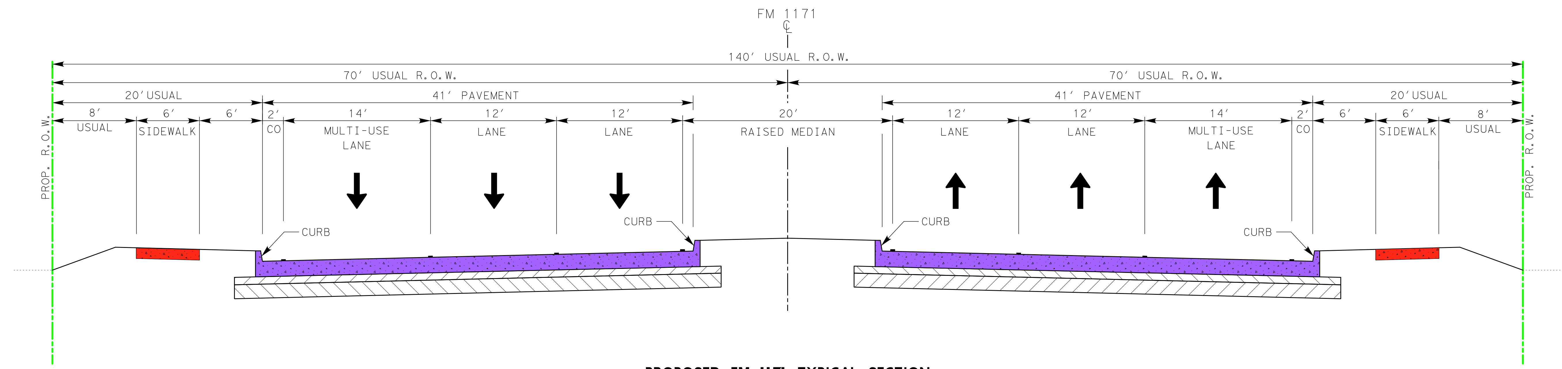
PROPOSED FM 1171 TYPICAL SECTION CENTRE ST TO HARMONSON RD
