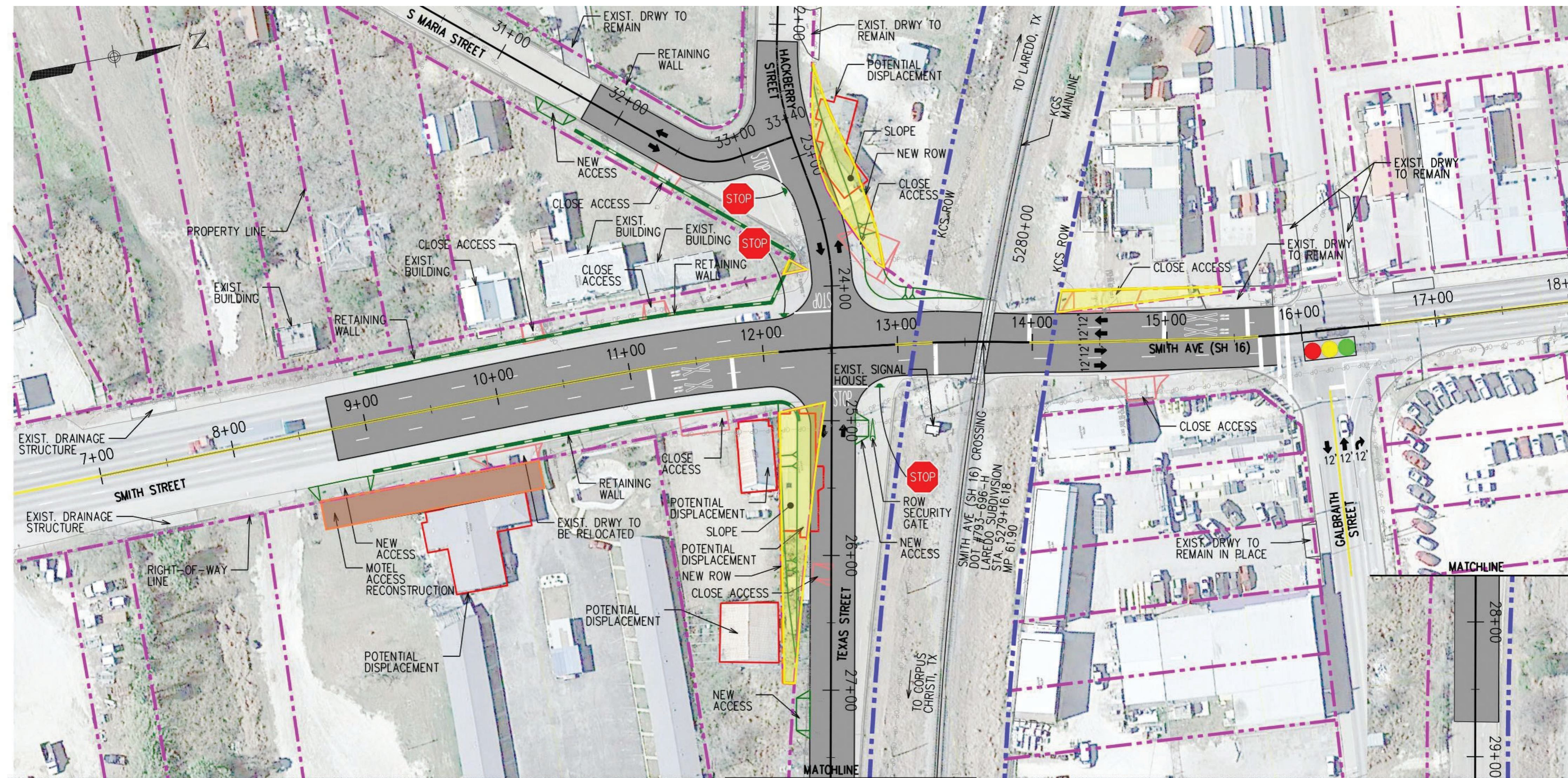
HBBR - Exhibit - Smith Xing - Alt. 1 Plan View
