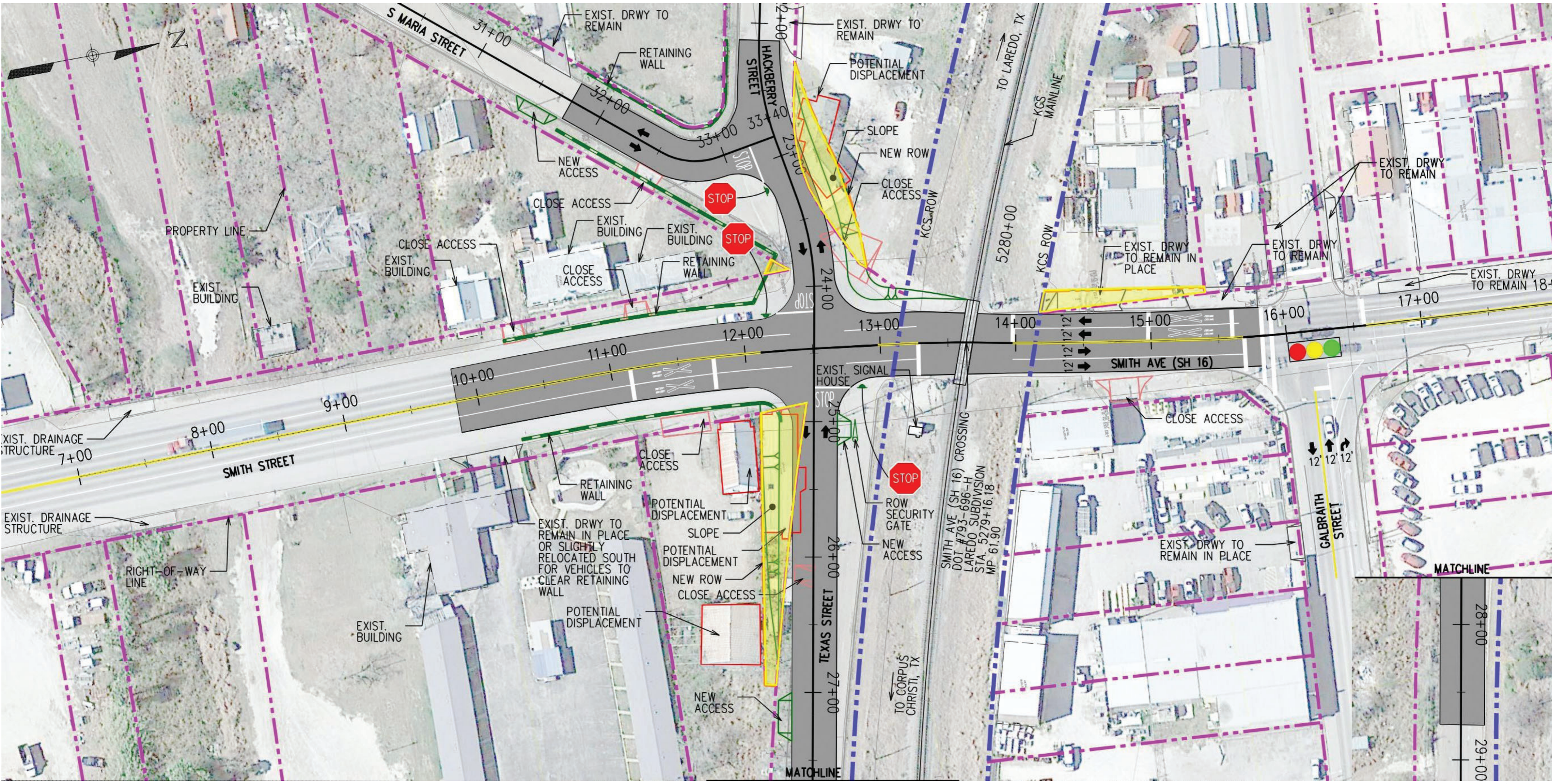
HBBR - Exhibit - Smith Xing - Alt. 2A Plan View
