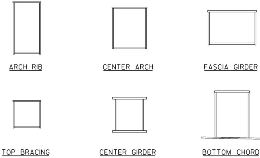
Figure 3: Typical Arch and Girder Sections
