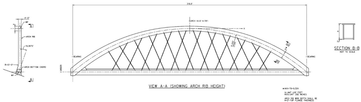
Figure 2: Arch Framing Geometry
