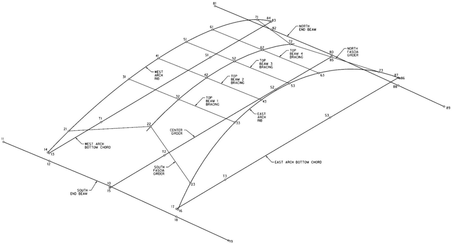
Figure 1: Bridge Frame
