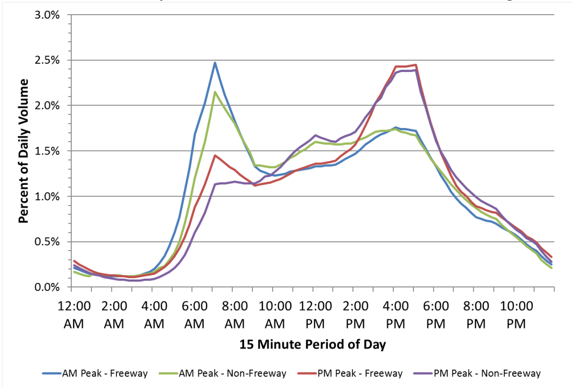
Exhibit A-1. Weekday Mixed-Traffic Distribution Profile for No to Low Congestion
