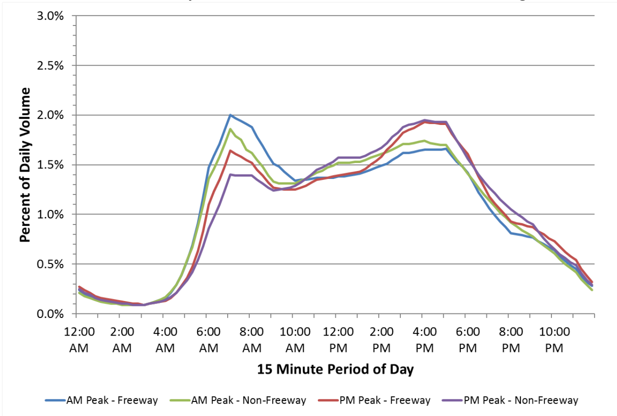
Exhibit A-3. Weekday Mixed-Traffic Distribution Profile for Severe Congestion
