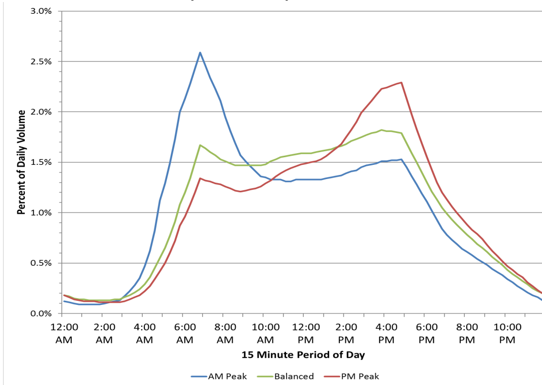
Exhibit A-8. Weekday Non-Freeway Truck-Traffic Distribution Profiles
