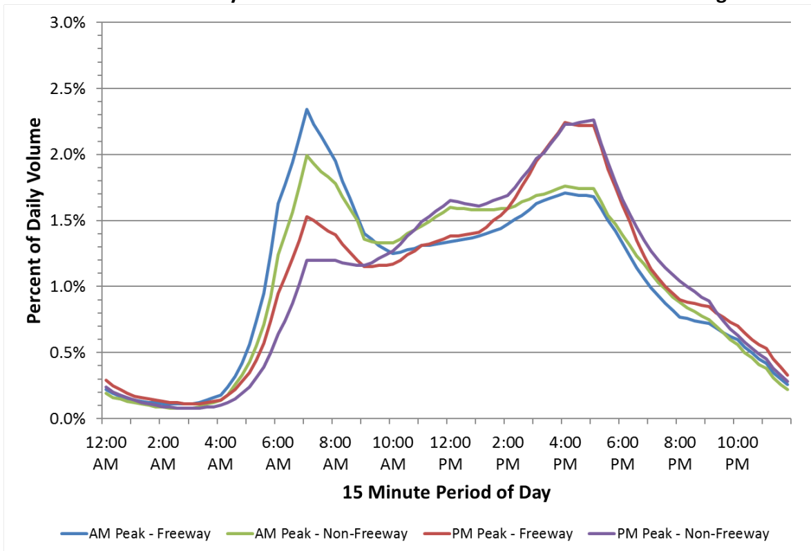
Exhibit A-2. Weekday Mixed-Traffic Distribution Profile for Moderate Congestion
