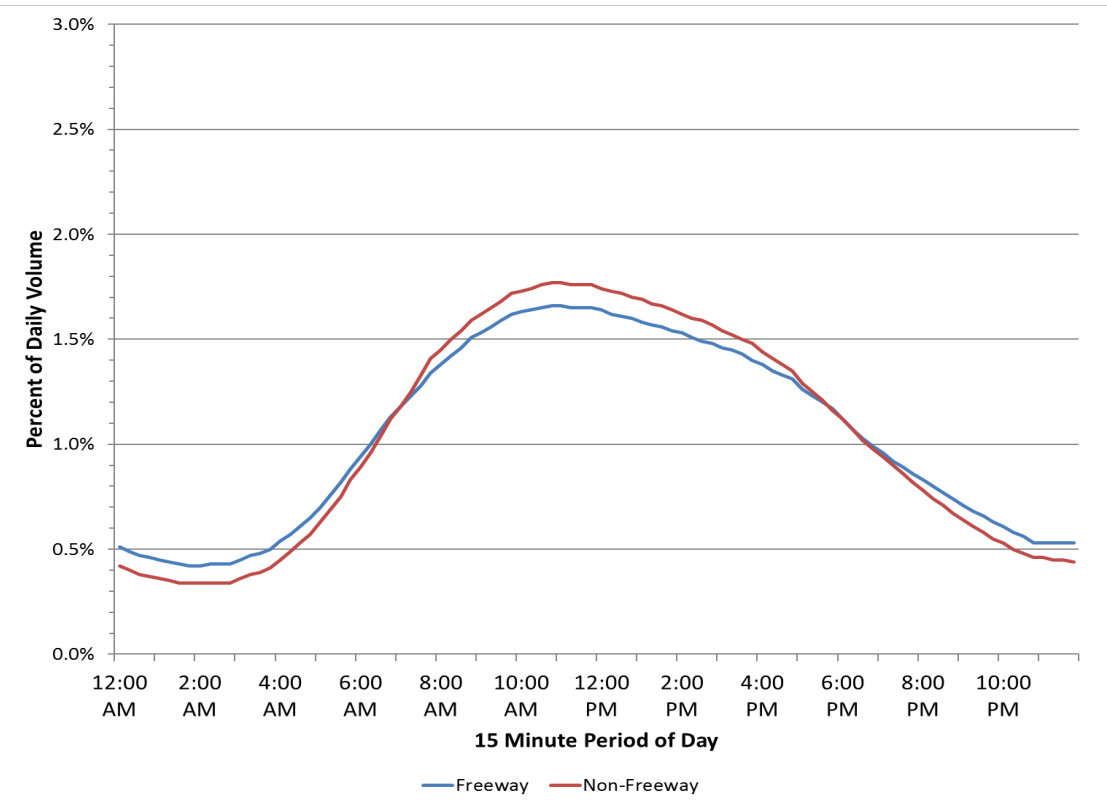
Exhibit A-9. Weekend Truck-Traffic Distribution Profiles
